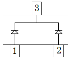
BAS40WT-05Q Marking:45
