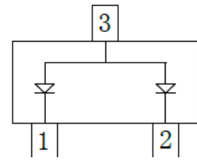
BAS40WT-06Q Marking:46
